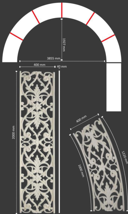
▲ PU-DKP-153
